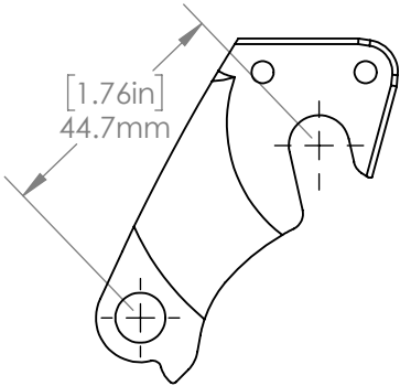
SHIMANO DIRECT MOUNT HANGER MOUNTAIN B4134, DR4134
