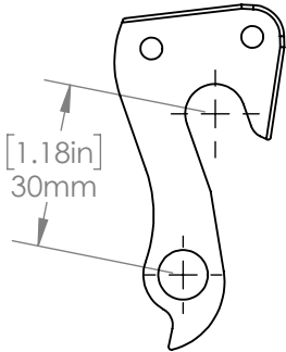
LONG HANGER B4101, DR4101 DR2061 (STEEL)
