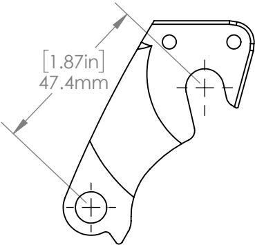
SHIMANO DIRECT MOUNT HANGER ROAD B4135, DR4135
