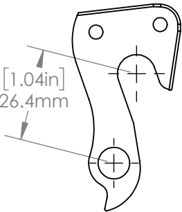
SHORT HANGER B4102, DR4102 DR2062 (STEEL)
