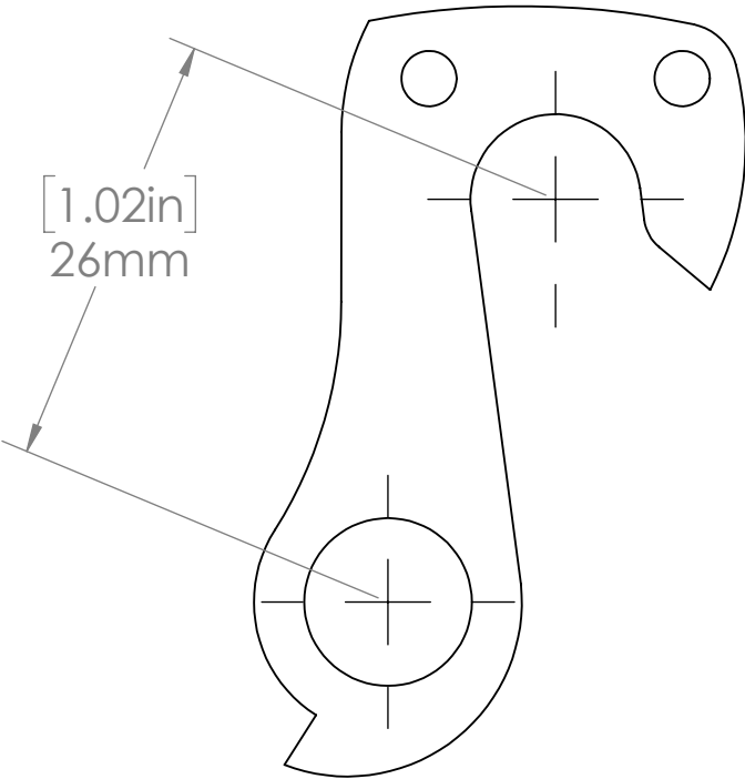
Short Hanger DR2064 (Steel) B4120, DR4120 (2024 Al)
