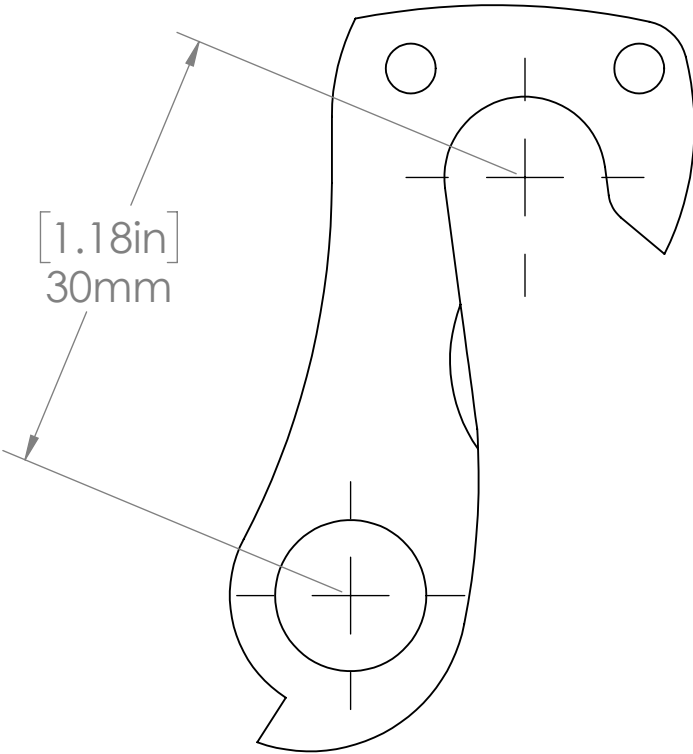
Long Hanger DR2063 (Steel) B4121, DR4121 (2024 Al)
