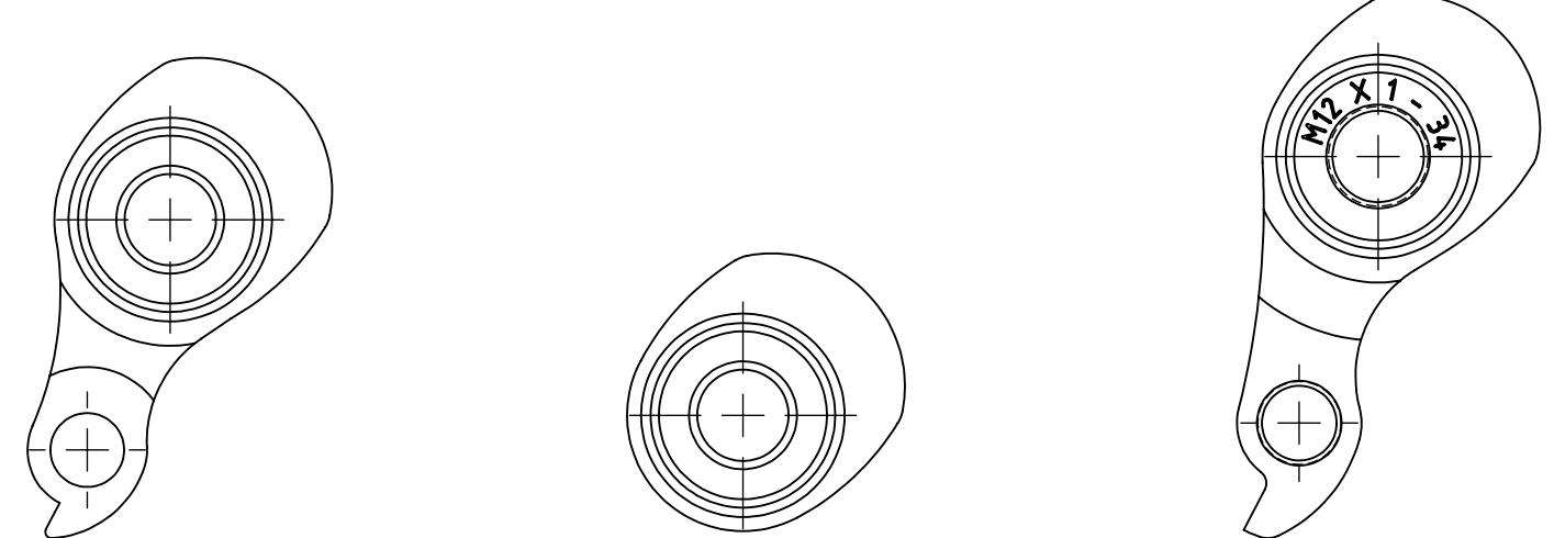
B4038 / DR4038 DT SWISS 12 mm HANGER
